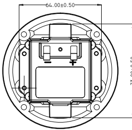
Mechanical drawing
