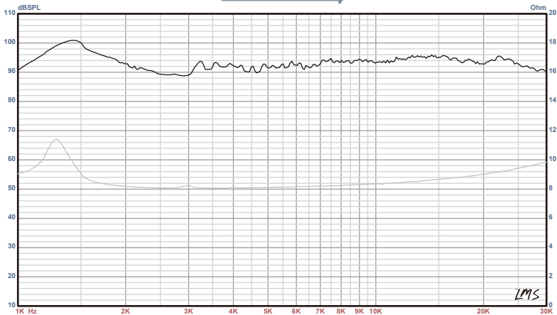
on-axis frequency response
