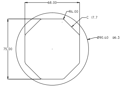
Recommand Cutout
